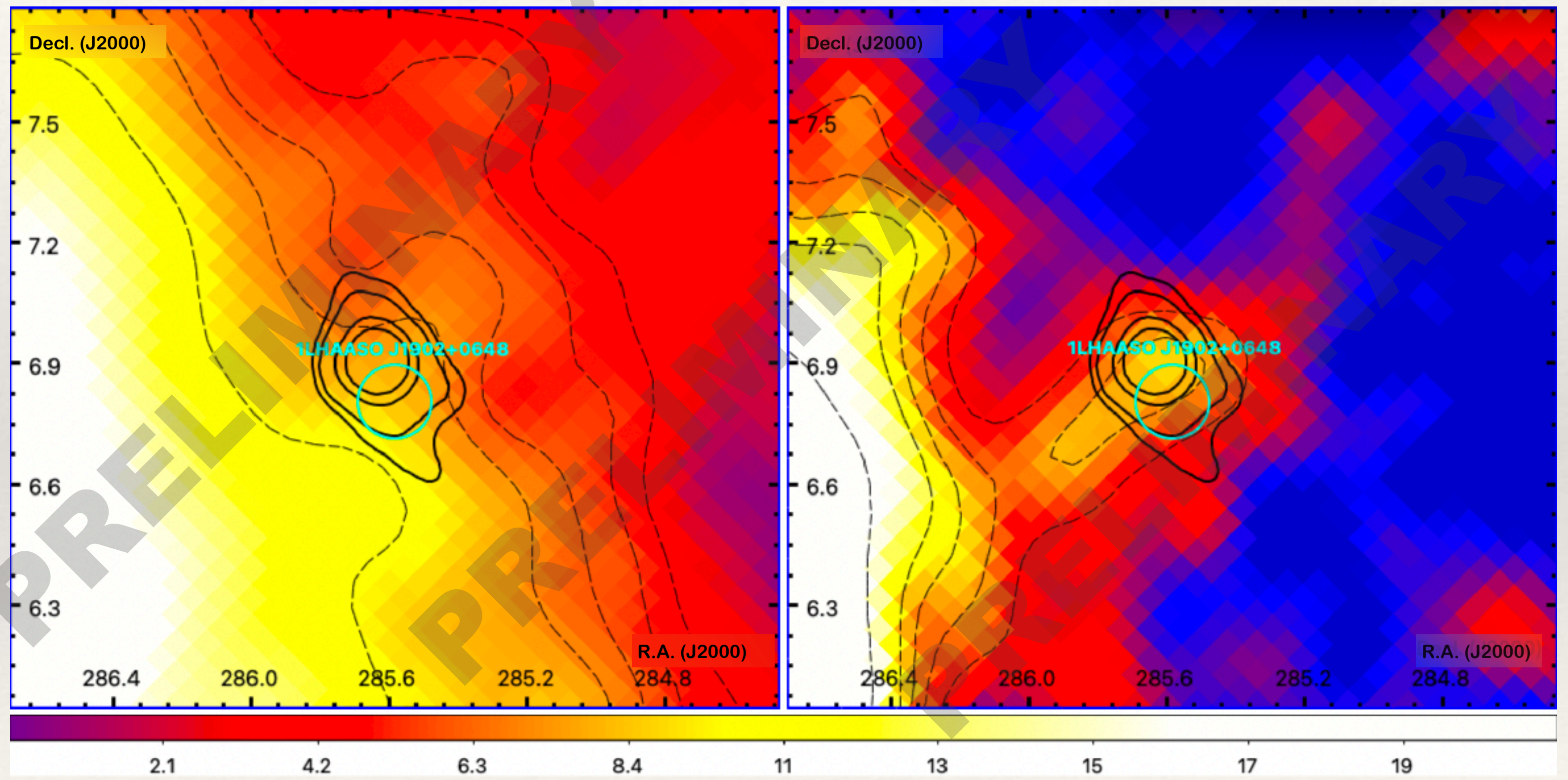
TeV Gamma Rays ( E < 10 TeV) TeV Gamma Rays ( E > 10 TeV)
