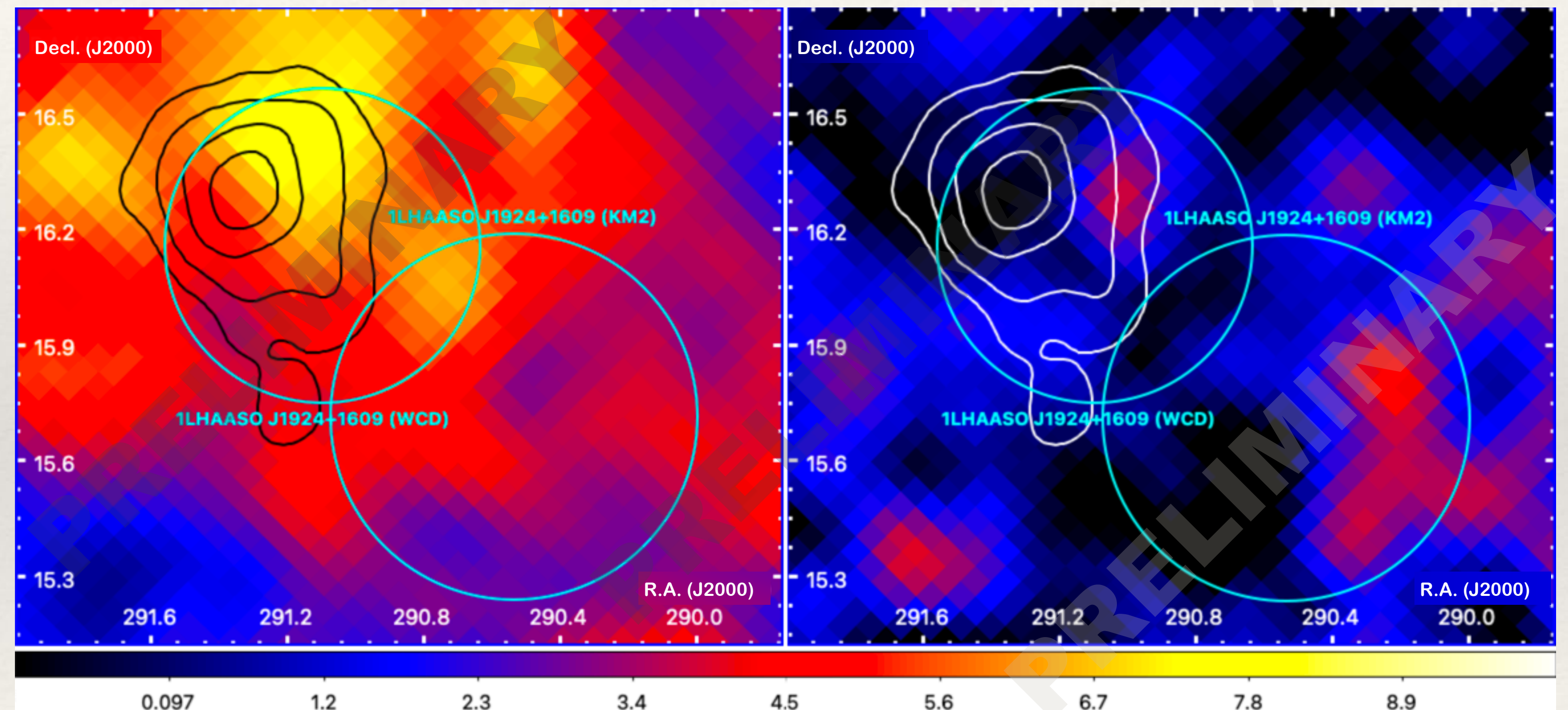
1LHAASO J1924+1609 (G51.26+0.11 & 4FGL J1925.2+1600c)
